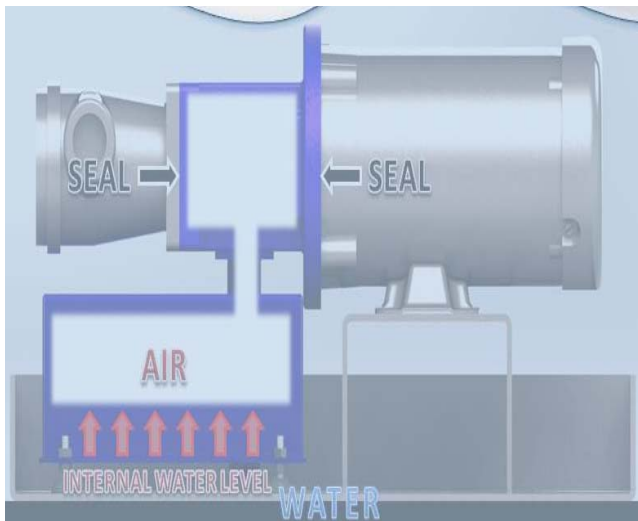
Flooded: The ESB is engineered to maintain an air reservoir to protect shaft seals and couplings from contact with water
